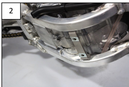
2 Put the front bracket in place Mettre la bride en place
